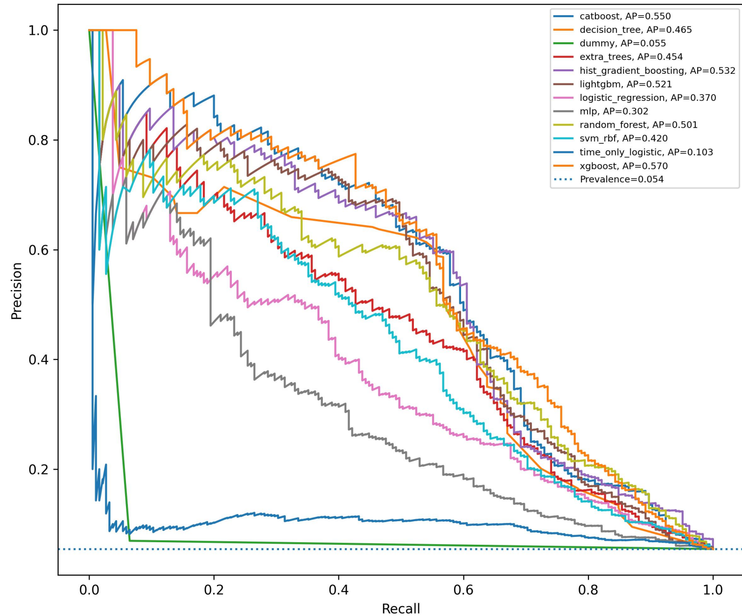
Precision recall curves
